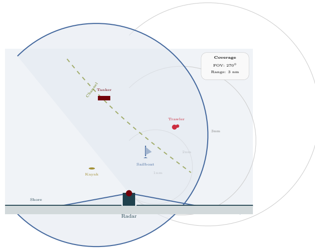
Figure 5: Radar installation geometry. The shore-mounted radar covers a 270° arc over Charleston Harbor, capturing vessels from kayaks at close range to tankers in the shipping channel.
