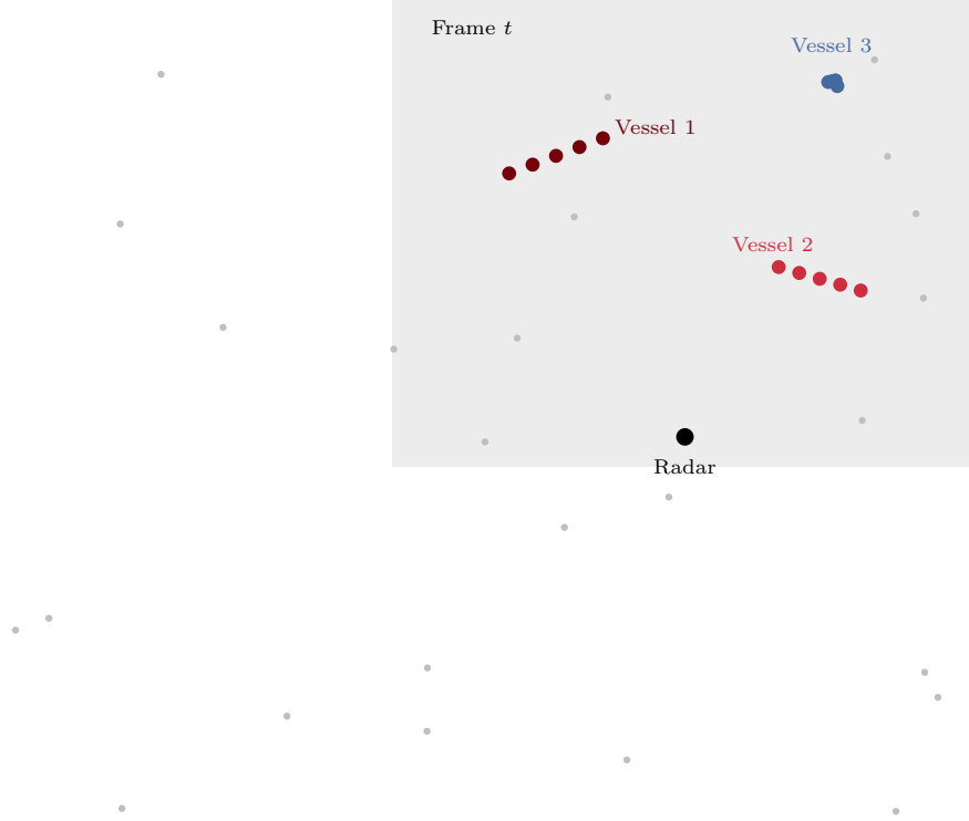
Figure 8: Example radar point cloud with three tracked vessels (colored) amid sea clutter (gray). Each cluster represents a distinct vessel identity maintained across frames.
