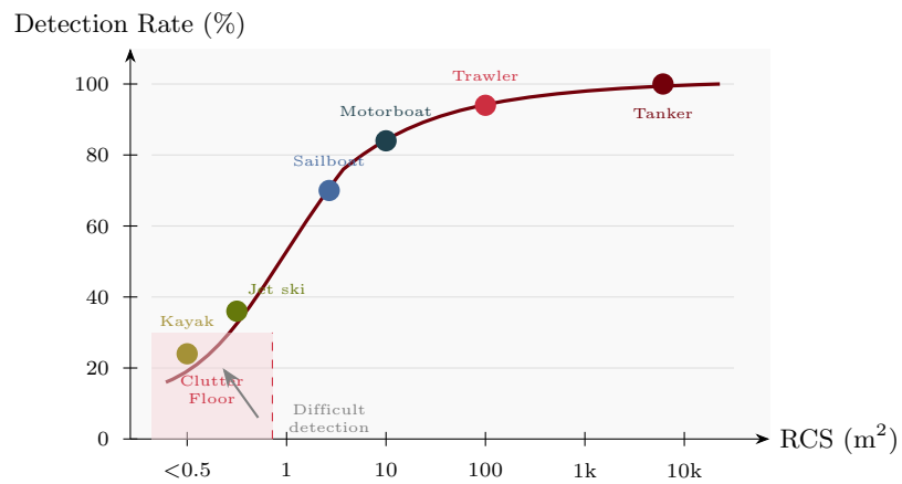
Figure 6: Detection rate versus radar cross-section (RCS). Small vessels with RCS below 1 m² operate near the sea clutter floor, resulting in intermittent detections. Larger vessels achieve near-perfect detection rates.
